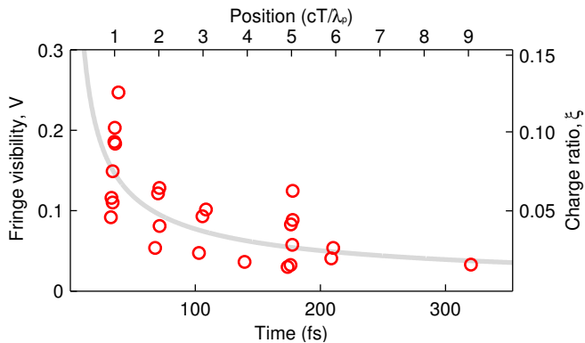
Figure 3. (Color online) Fringe visibility for sinusoidal oscillation that contained only one significant peak in the Fourier Transform, as function of the position of that peak. The charge ratio \xi = q_n/q_o is calculated from the visibility using Eq. 2 in the limit where both bunches have similar shapes and energy distributions. The measurements were performed using CPI for n_e = 10 \times 10^{18} \text{ cm}^{-3} .
