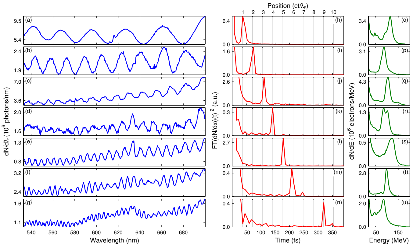
Figure 1. (Color online) Selected and sorted examples of sinusoidal CTR modulations, obtained using CPI for n_e = 10 \times 10^{18} \text{cm}^{-3} and \lambda_p = 10.6 \mu\text{m} . Three panels on each row represent one measurement. (a–g): CTR spectra. (h–n): Square amplitude of the Fourier transform of the CTR spectra. (o–u): Corresponding electron spectra.
