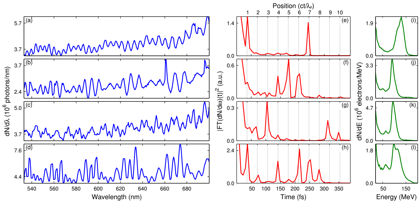
Figure 2. (Color online) Selected examples of complex CTR modulations, obtained using CPI for n_e = 10 \times 10^{18} \text{ cm}^{-3} and \lambda_p = 10.6 \text{ }\mu\text{m} . Three panels on each row represent one measurement. (a–d): CTR spectra. (e–h): Fourier transform of the CTR spectra. (i–l): Corresponding electron spectra.
