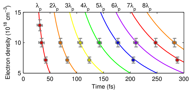
Figure 4. (Color online) Average positions of the Fourier peaks for different plasma densities (o) are compared to multiples of the plasma wave period (lines). Horizontal errorbars denote the standard deviation over the complete dataset. Vertical errorbars is an estimate of the uncertainty in plasma density.
