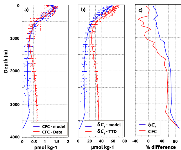
Figure 5. Comparison of average vertical profiles along the Meteor M51/2 section for (a) CFC-12 (pmol kg -1 ), (b) δC T (μmol kg -1 ), and (c) the model–data relative difference (in percent). Model results are in blue, while red indicates the CFC-12 data and δC T data-based estimates; the right panel (c) uses blue for δC T and red for CFC-12. Data-based estimates for δC T are the TTD results from Schneider et al. (2010).
