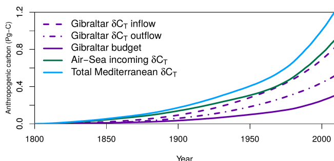
Figure 7. Cumulative increase in anthropogenic carbon (Pg C) in the Mediterranean Sea from 1800 to 2008 due to the Gibraltar inflow (dashed purple line) and outflow (dashed-dotted purple line), i.e., their difference (inflow – outflow, solid purple line) and the air–sea flux (solid green line). Also shown is the total buildup in storage (solid light-blue line). Gibraltar fluxes have been calculated from model monthly mean outputs by multiplying the anthropogenic carbon concentration ( \text{g m}^{-3} ) of water in a section crossing the Strait of Gibraltar by water fluxes ( \text{m}^3 \text{ month}^{-1} ) flowing across this section. The sign of the water flux indicates its direction, and hence provides an inflow or an outflow of anthropogenic carbon. The total storage is the sum of the net \delta C_T flux at the Strait of Gibraltar and of the \delta C_T air–sea flux, and is consistent with the sum of all the \delta C_T store in the Mediterranean Sea.
